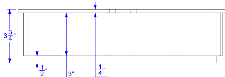
BASE TRAY - ELEVATION
