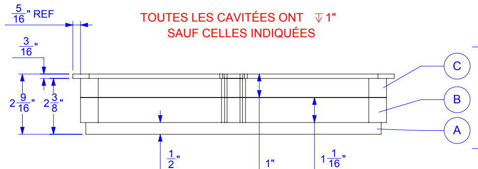
BASE TRAY - ELEVATION
