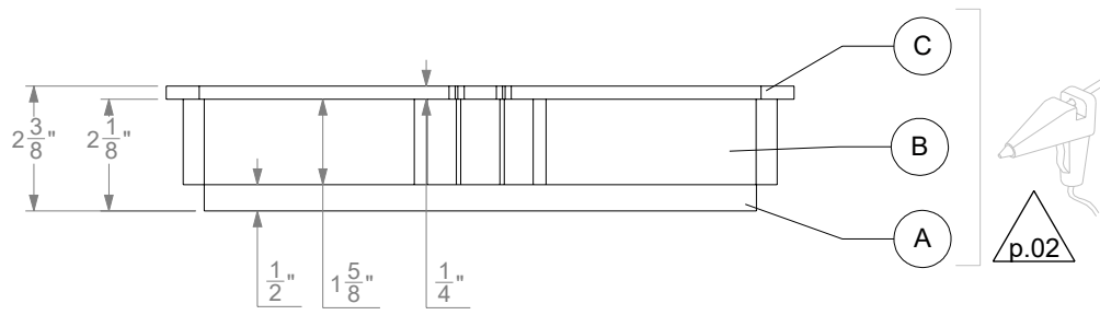
BASE TRAY - ELEVATION
