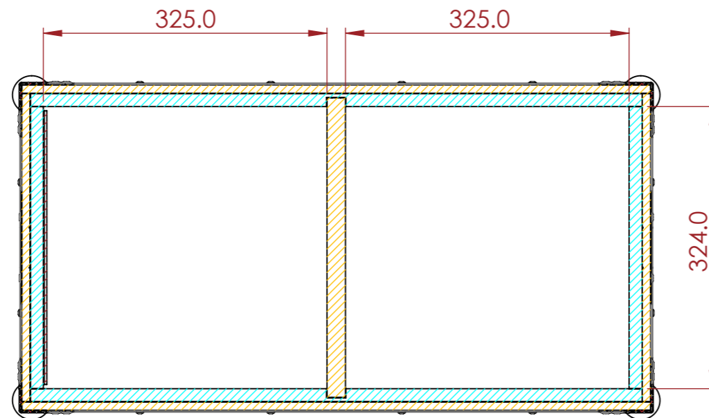
SECTION B-B
