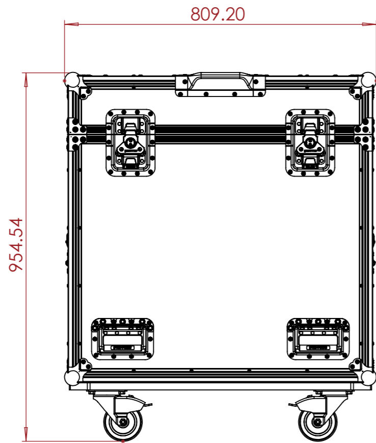
FROT VIEW
