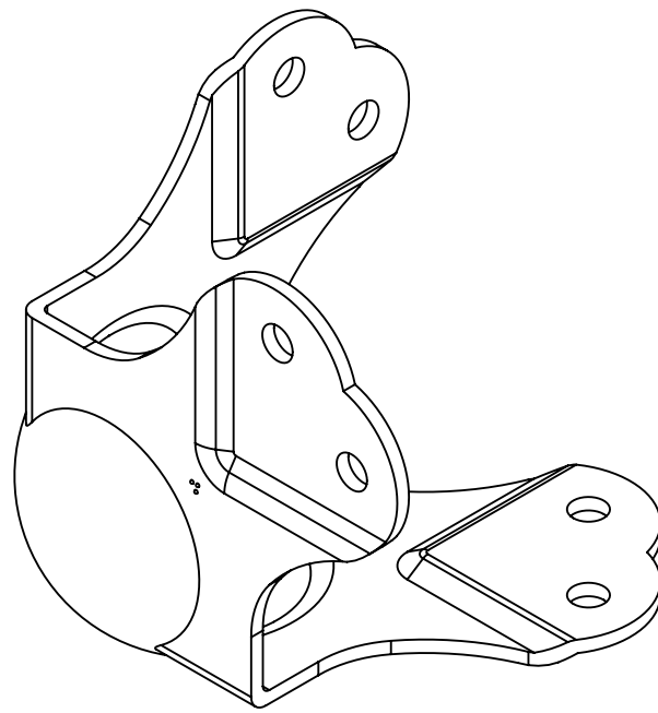
ISOMETRIC VIEW
