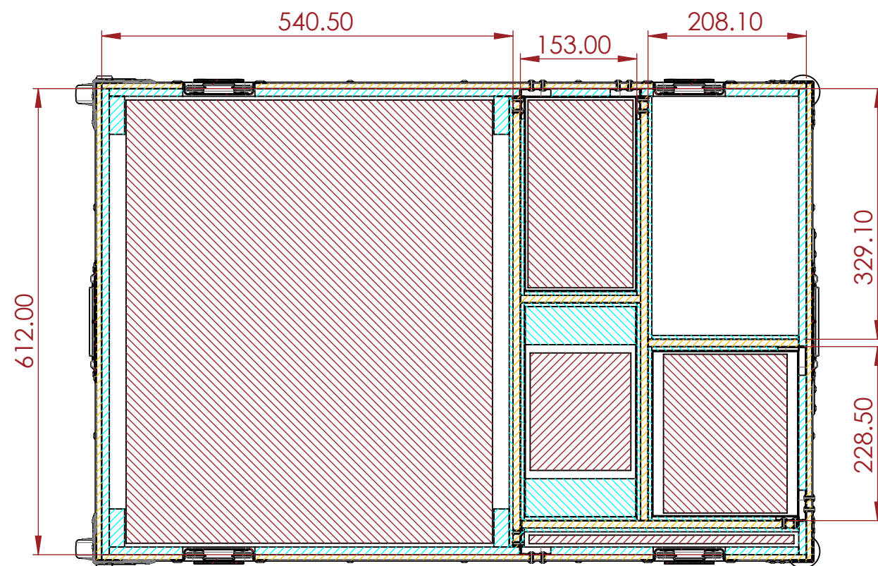
SECTION B-B
