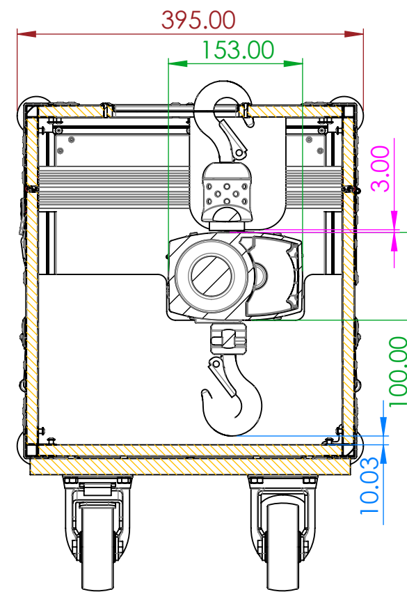
SECTION B-B
