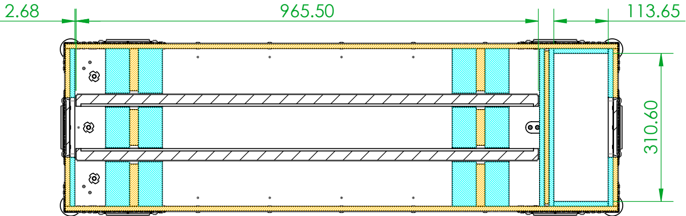
SECTION B-B
