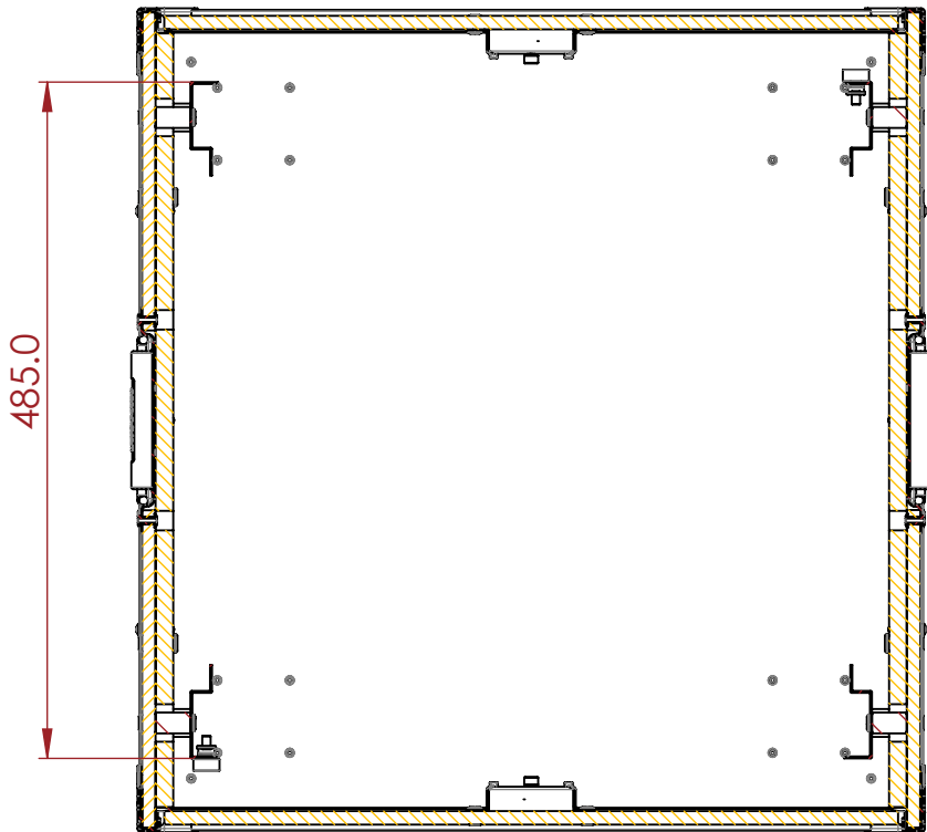
SECTION G-G
