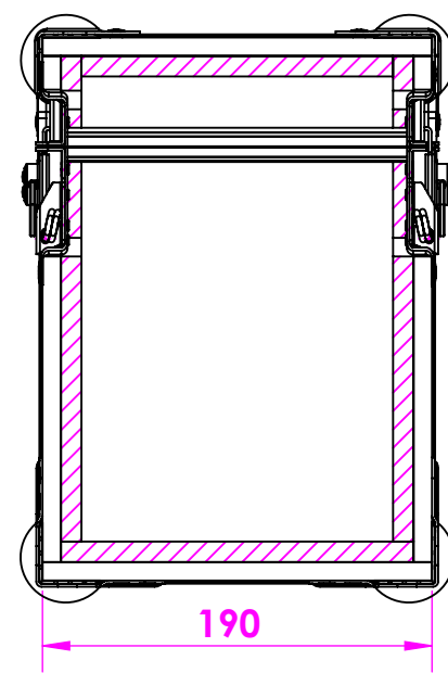
Side Cutout View
