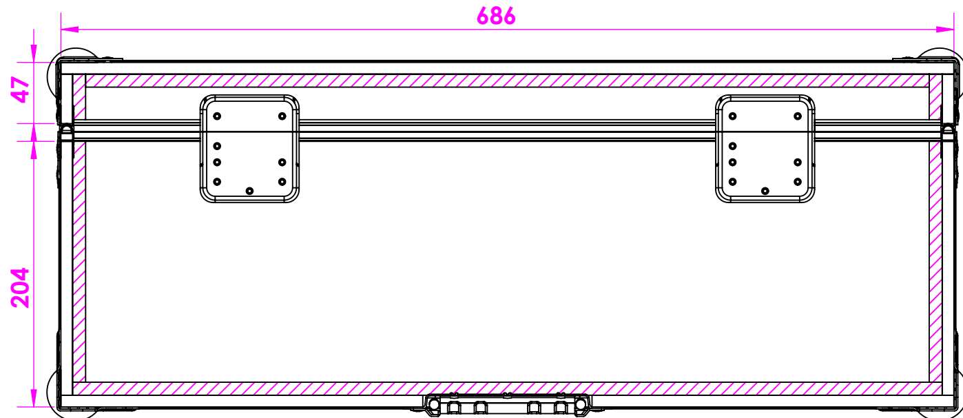
Front Cutout View
