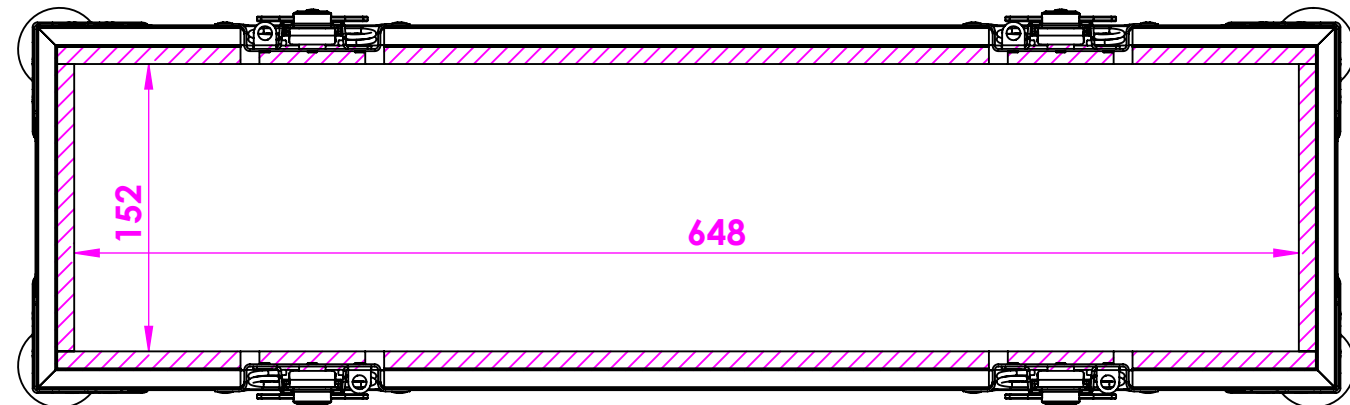
Top Cutout View
