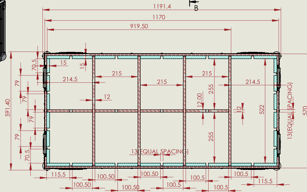
SECTION C-C
